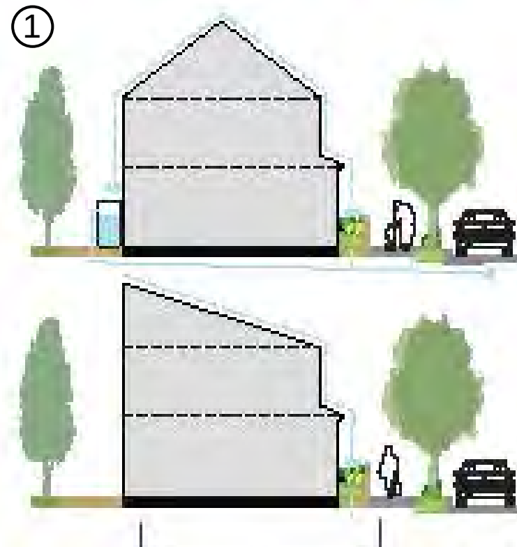
Roof drainage and SuDS options
